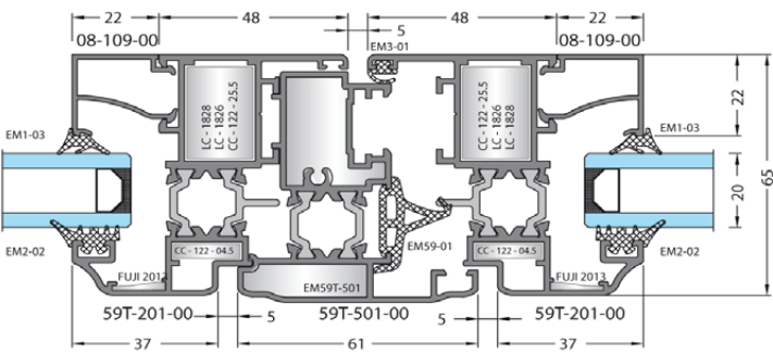
aluminium details
