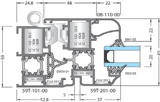
aluminium details
