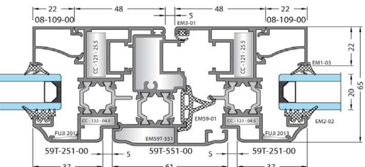
perimetric details
