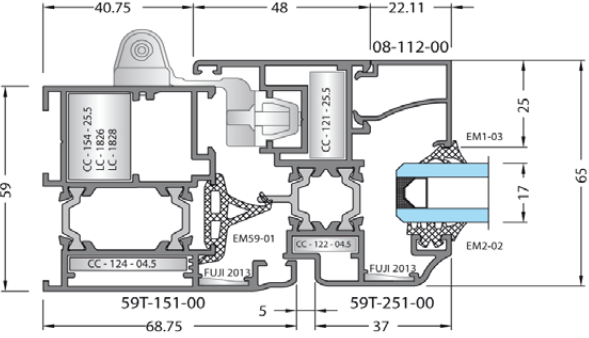
perimetric details
